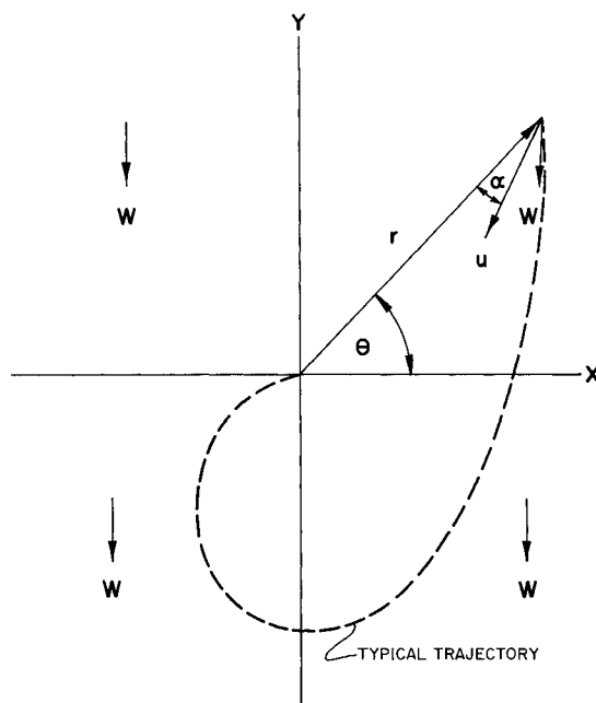
Fig. 1 Kinematics of azimuth homing.
